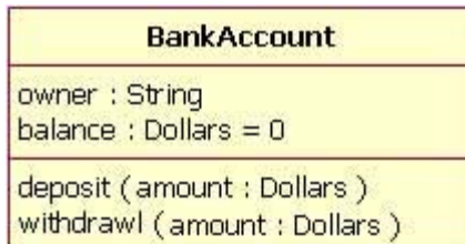
Figure 2: A Bank Account class diagram showing the balance attribute's value defaulted to zero dollars.
