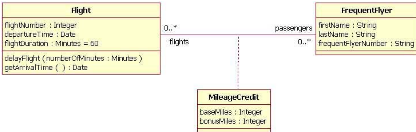
Figure 11: Adding the association class MileageCredit
