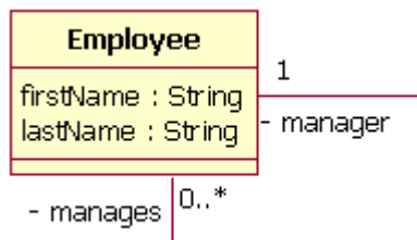
Figure 14: Example of a reflexive association relationship
