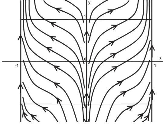
Figure 1: The flow \phi tangent to the vector field X .
