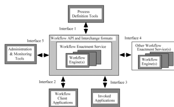
Figure 4 - The Workflow Reference Model
