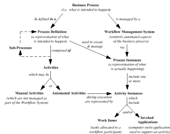
Figure 1 - Relationships between basic terminology
