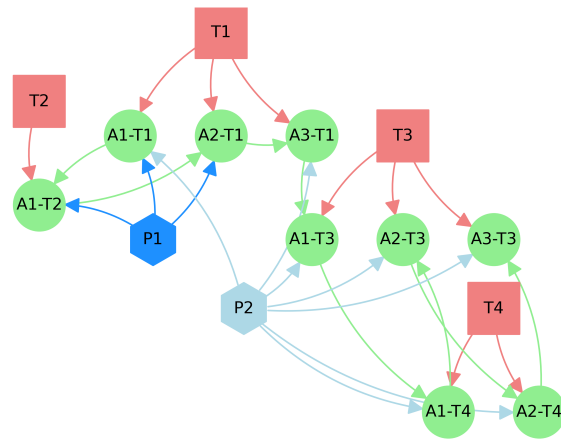
Fig. 3. Example for the proposed LQN-based graph model.
