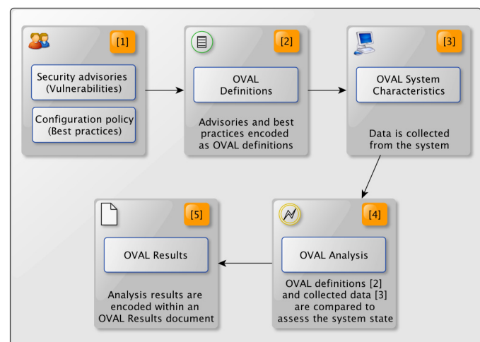
Fig. 7: OVAL-based vulnerability assessment [43]
